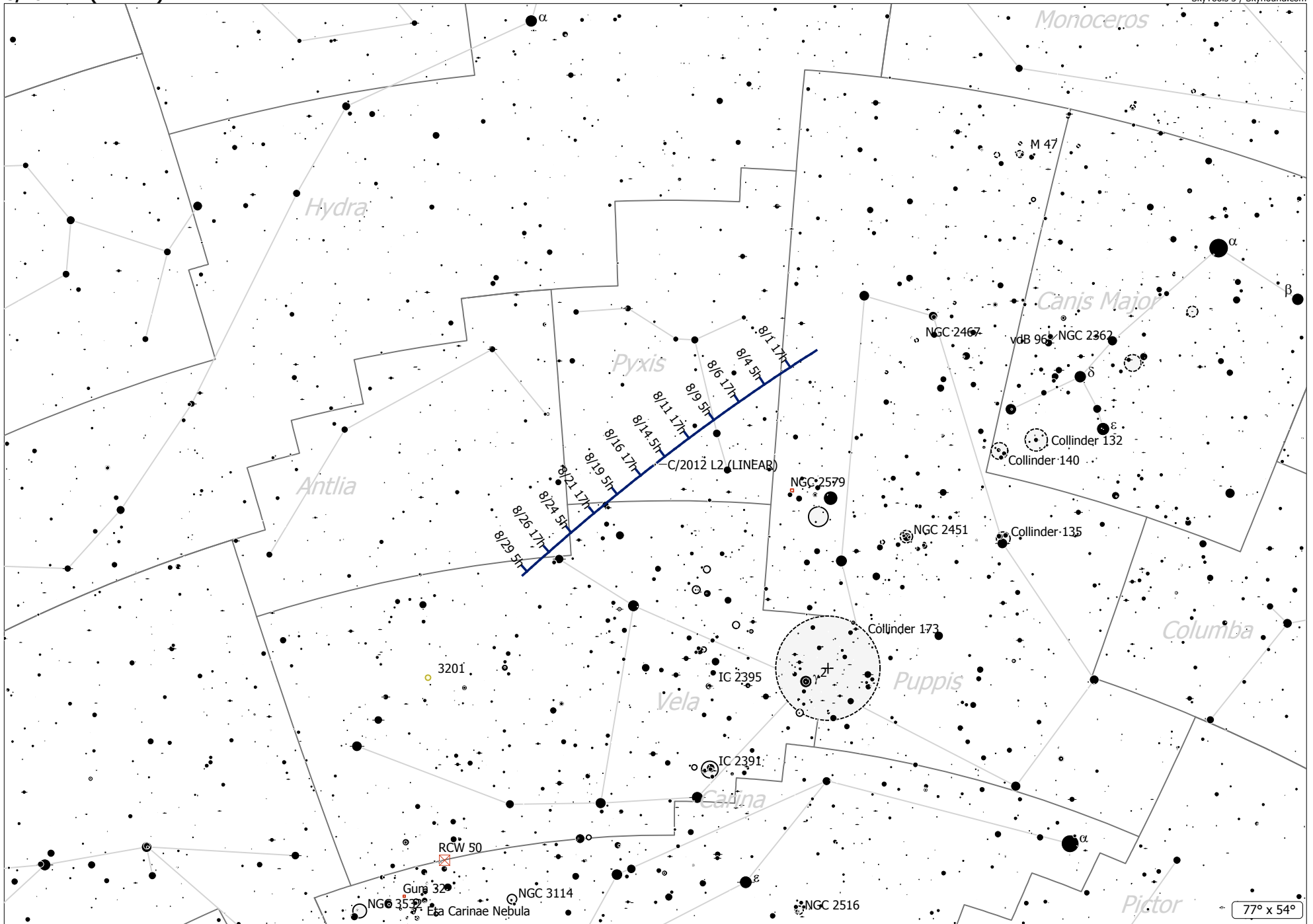
C/2012 L2 (LINEAR) (Comet) Magnitude: 12.11 Coma Diameter: 1.4' SBR: 21.5 Mag/arcsec 2 Earth
