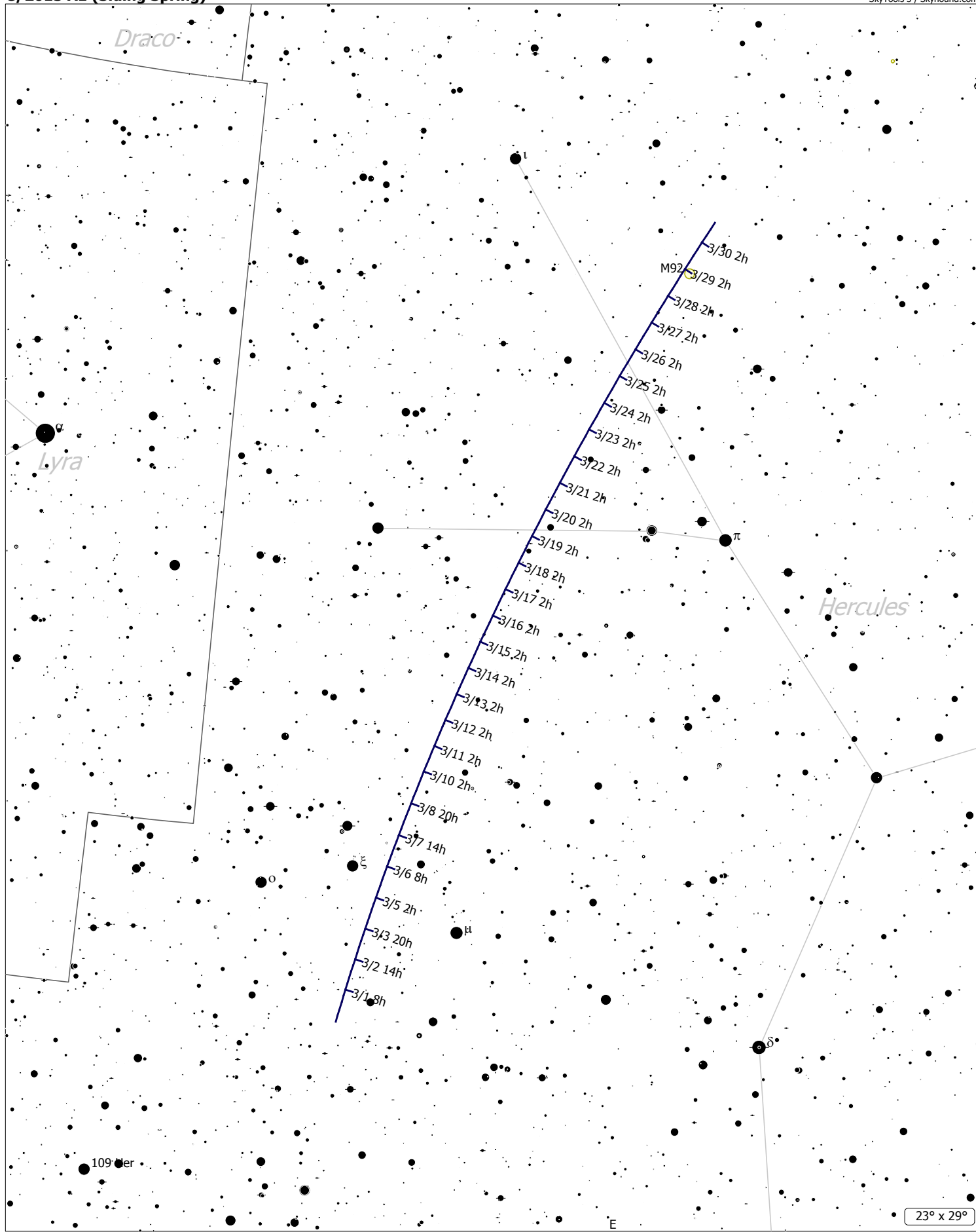
C/2013 A1 (Siding Spring) (Comet) Magnitude: 12.08 Coma Diameter: 2.3' SBR: 22.5 Mag/arcsec 2 Earth
