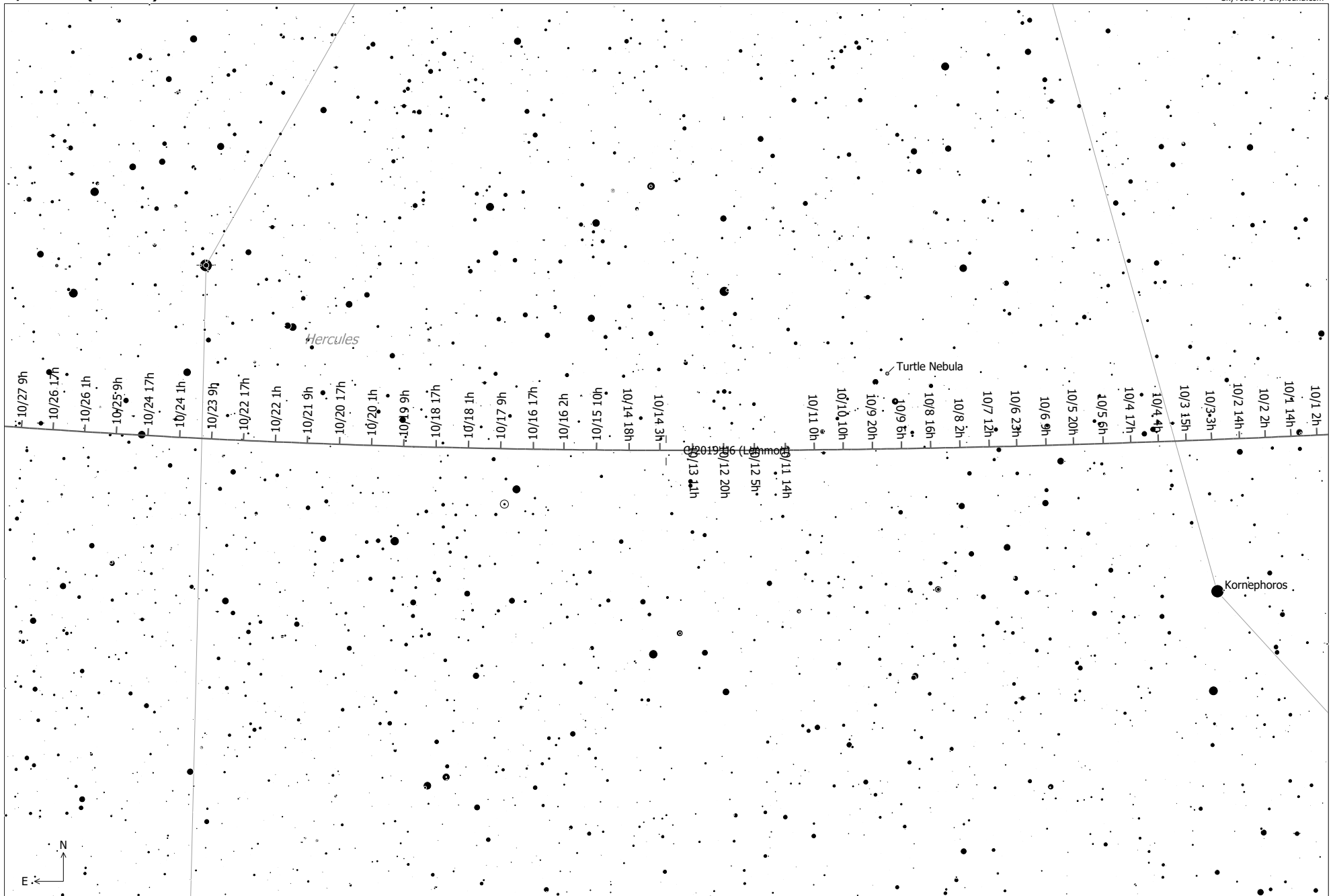
C/2019 U6 (Lemmon) (Comet)
