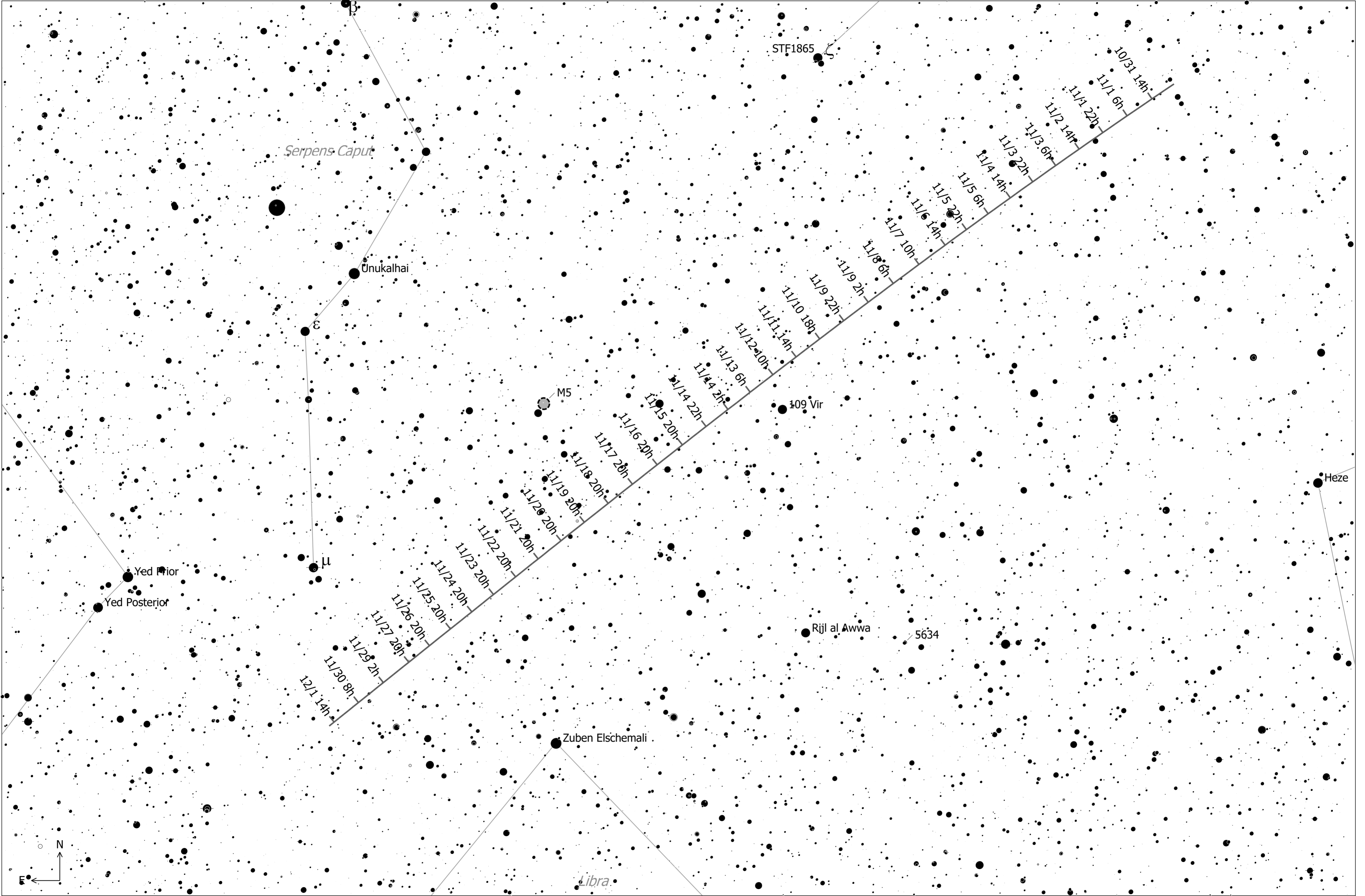
C/2022 R2 (ATLAS) (Comet) Magnitude: 14.30 Coma Diameter: 51" SBr: 22.6 Mag/arcsec 2 Earth Distance: 1.6 AU
