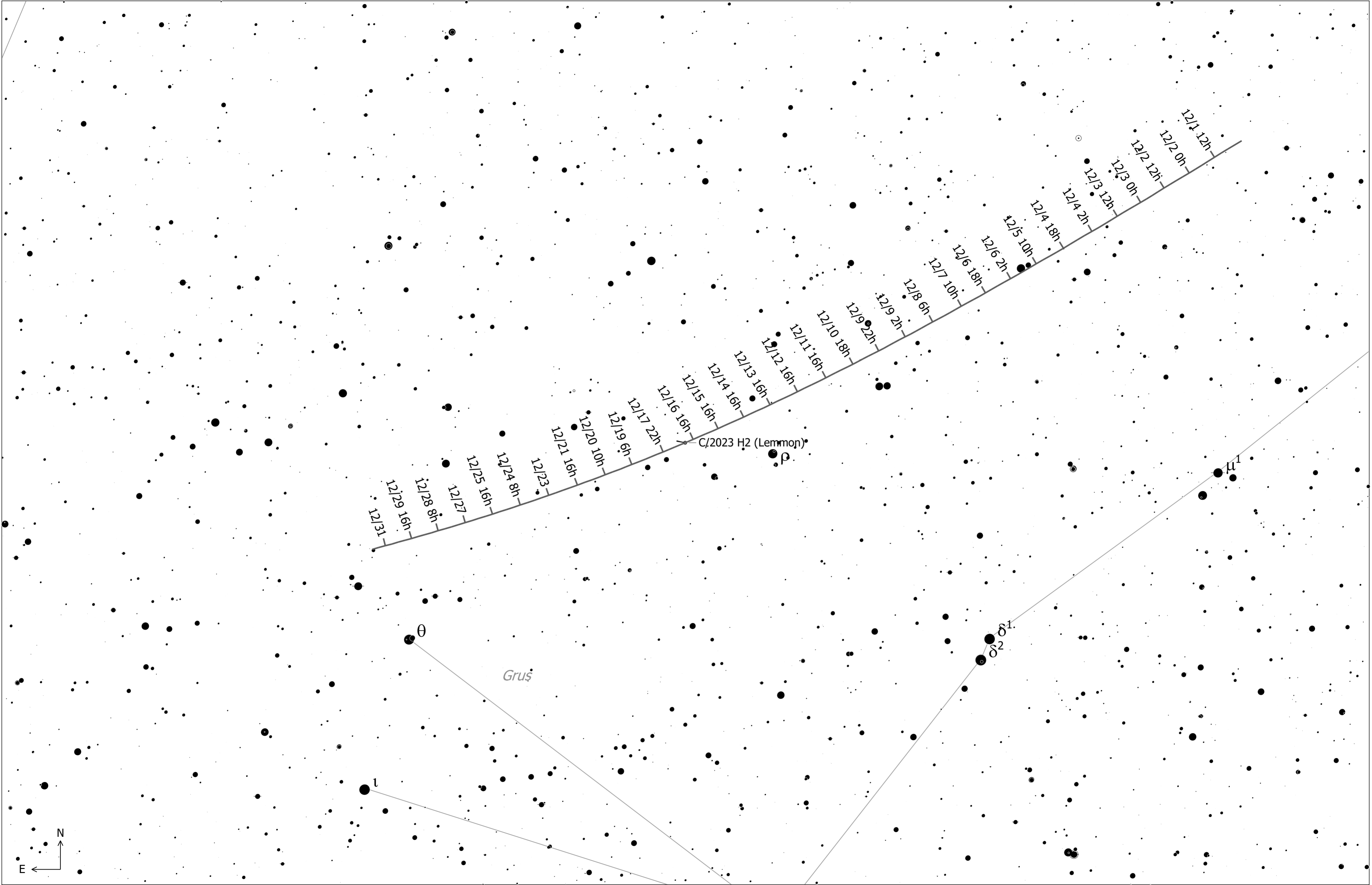
C/2023 H2 (Lemmon) (Comet) Magnitude: 11.58 Coma Diameter: 2.2' SBr: 21.9 Mag/arcsec 2 Earth Distance: 1.2 AU
