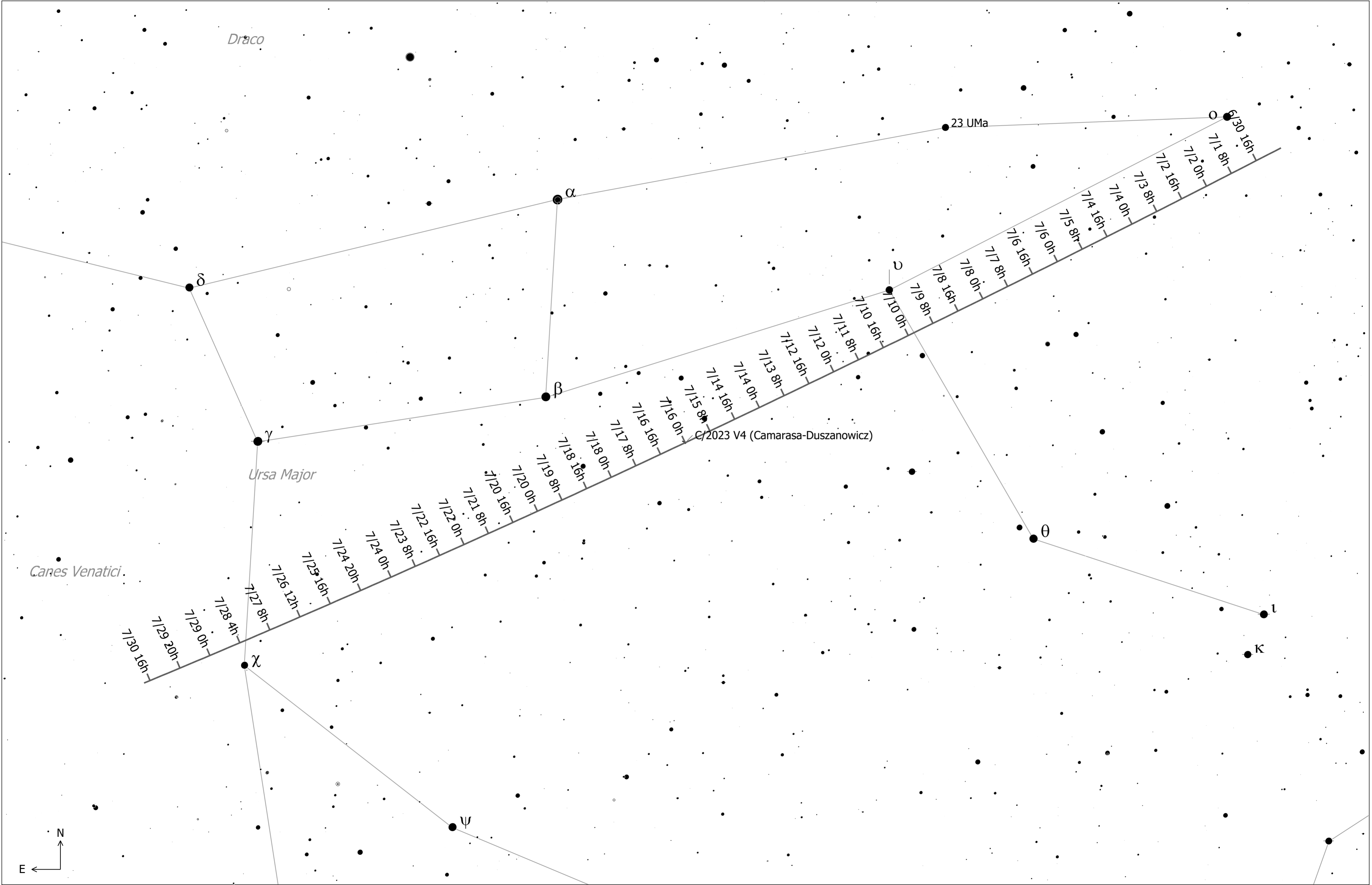
C/2023 V4 (Camarasa-Duszanowicz) (Comet) Magnitude: 11.78 Coma Diameter: 2.9' SBr: 22.7 Mag/arcsec 2 Earth Distance: 1.8 AU
