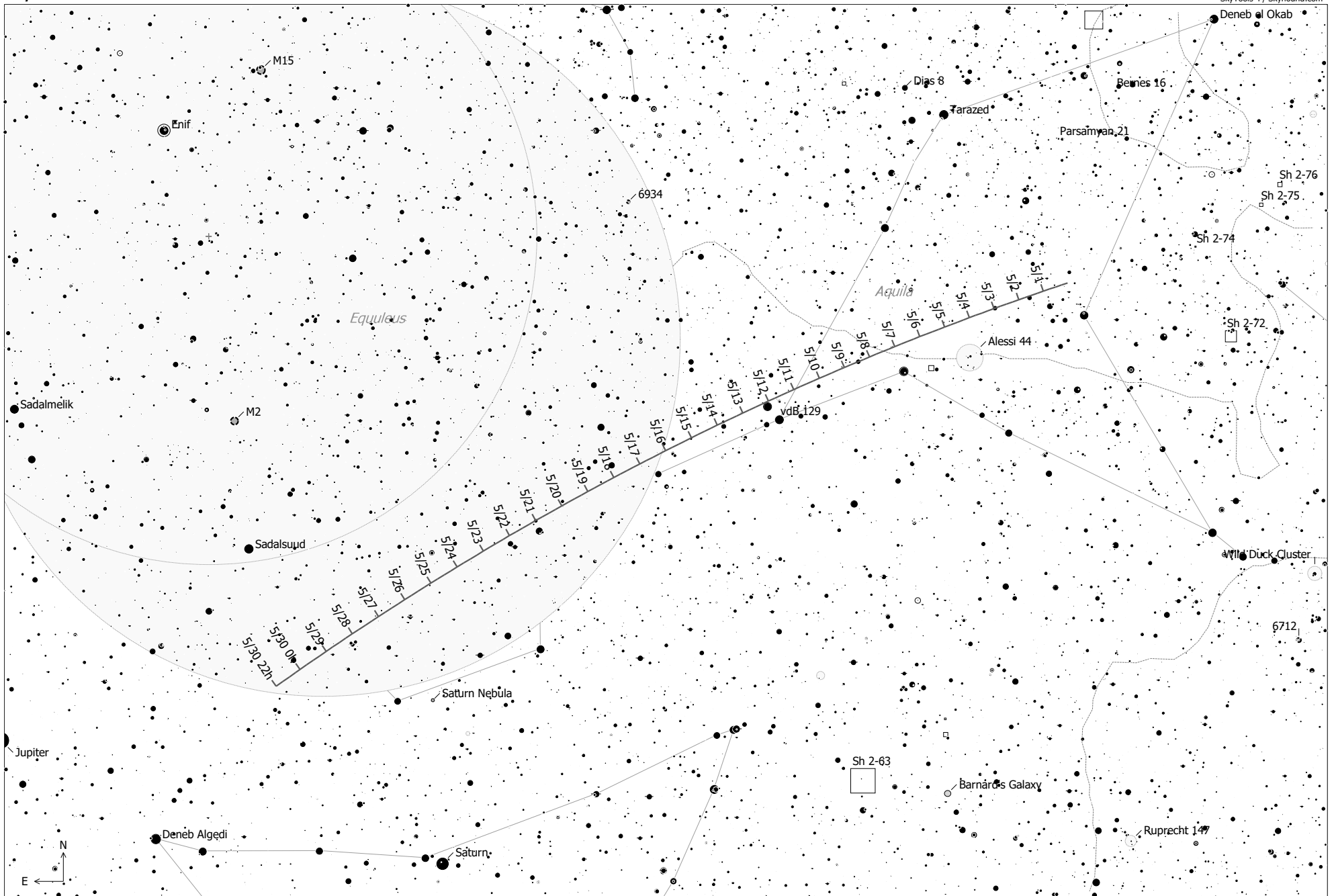
7P/Pons-Winnecke (Comet) Magnitude: 12.19 Coma Diameter: 4.5' SBr: 24.1 Mag/arcsec 2 Earth Distance: 0.5 AU
